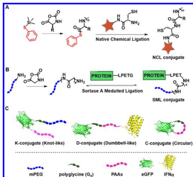
Figure 1. (A) Synthesis of poly(amino acid)s (PAAs) by phenyl trimethylsilyl sulfide (PhS-TMS)-mediated controlled ROP of NCAs. A thioester was installed to the C-terminus of the PAA and serves as a chemical handle for native chemical ligation (NCL). (B) A polyglycine ( G_x ) nucleophile was generated by the ROP of glycine NCA as a substrate for sortase A-mediated ligation (SML). (C) Illustration of various site-specific topological protein–PAA conjugates described in this work.
